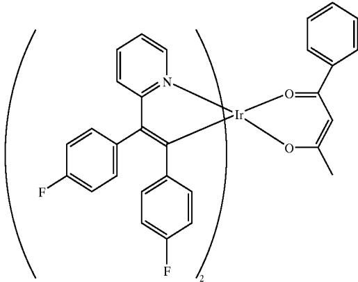
COMPOUND 13
