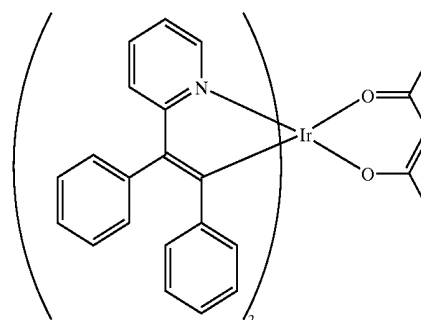
COMPOUND 2
