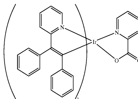
COMPOUND 10
