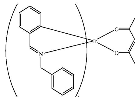
COMPOUND 11
